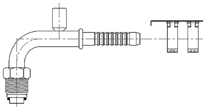
90 DEGREE MALE O-RING (MOR) WITH SWITCH OR SERVICE PORT
